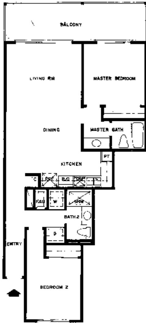
THE SANDPIPER · Plan 2A-3 Two Bedrooms Two Baths 1139 Sq Ft (including Private Balcony, excluding Carport)
